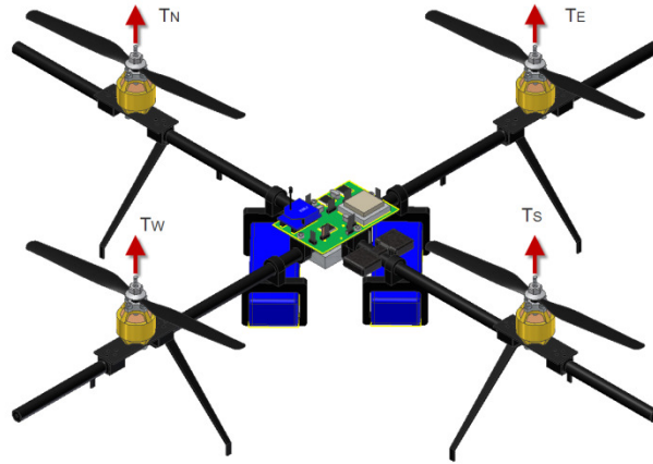
Figure 1: The Quadrotor Aerial Structure
