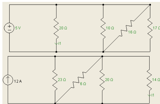
Figure 3: Circuit Tutor Examples
